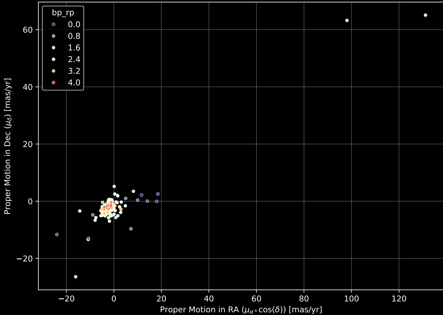
APOGEE DR17 Field: [Lac_3] Proper Motion Diagram (n= 147)
