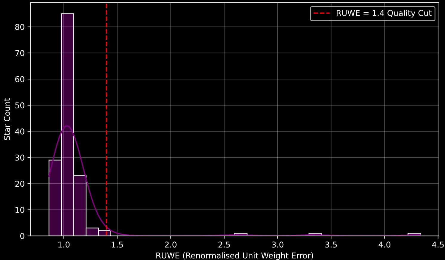
GAPOGEE DR17 Field [Lac_3] RUWE Distribution (n= 145)
