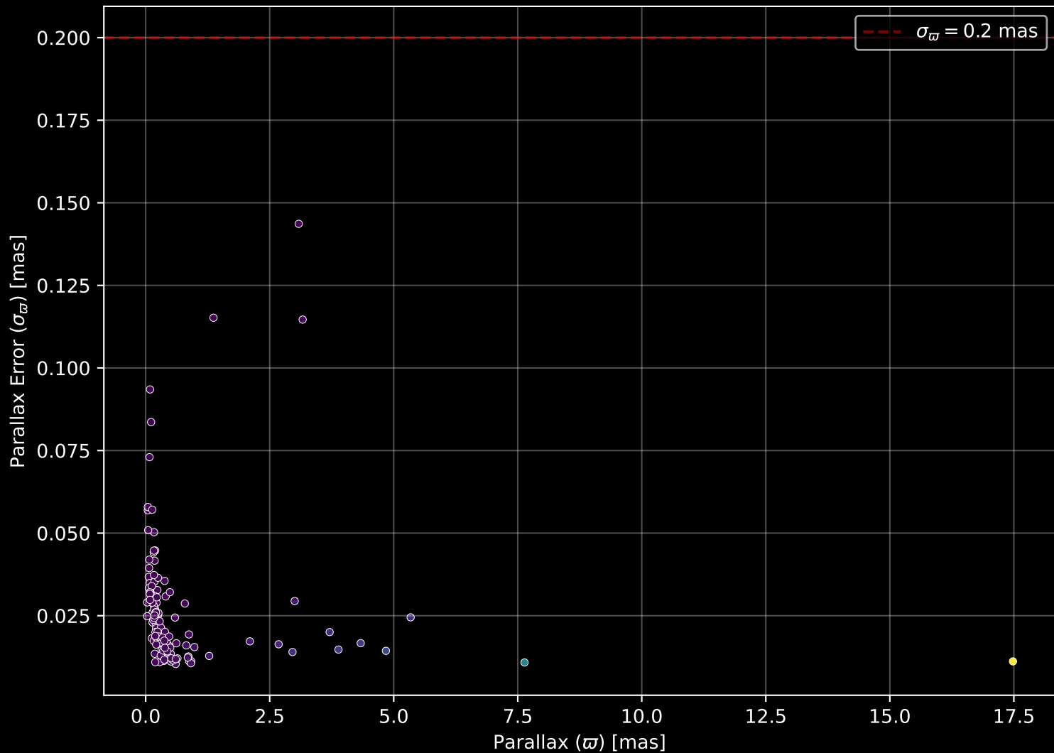
APOGEE DR17 Field: [Lac 3] Parallax Quality (n= 147)
