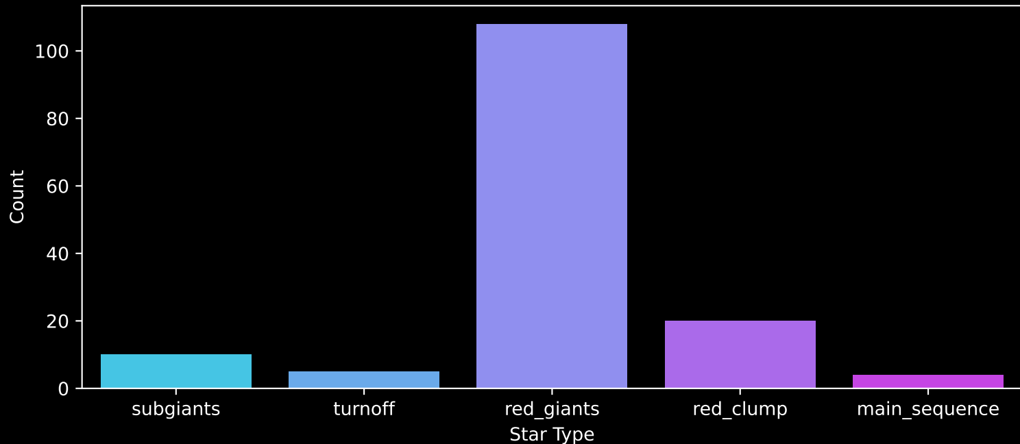
APOGEE DR17 Field: [Lac_3] Count plot of Star Type
