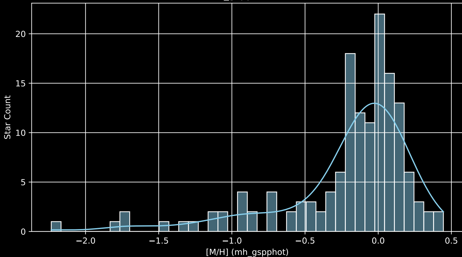
APOGEE DR17 Field: [Lac_3 [M/H] (mh_gspphot) (n= 146)
