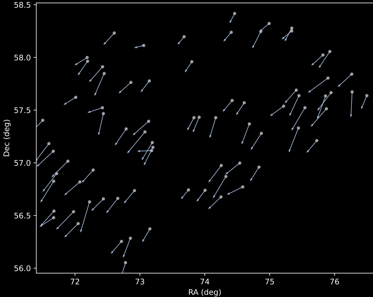
APOGEE DR17 Cluster 1 Proper Motion Vectors (n=75)
